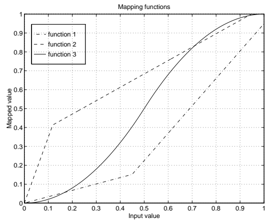
Figure 2: Mapping functions.
