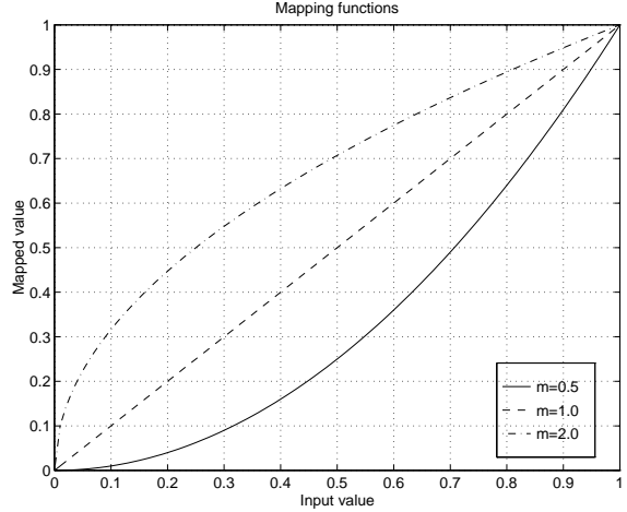
Figure 1: Mapping functions.
